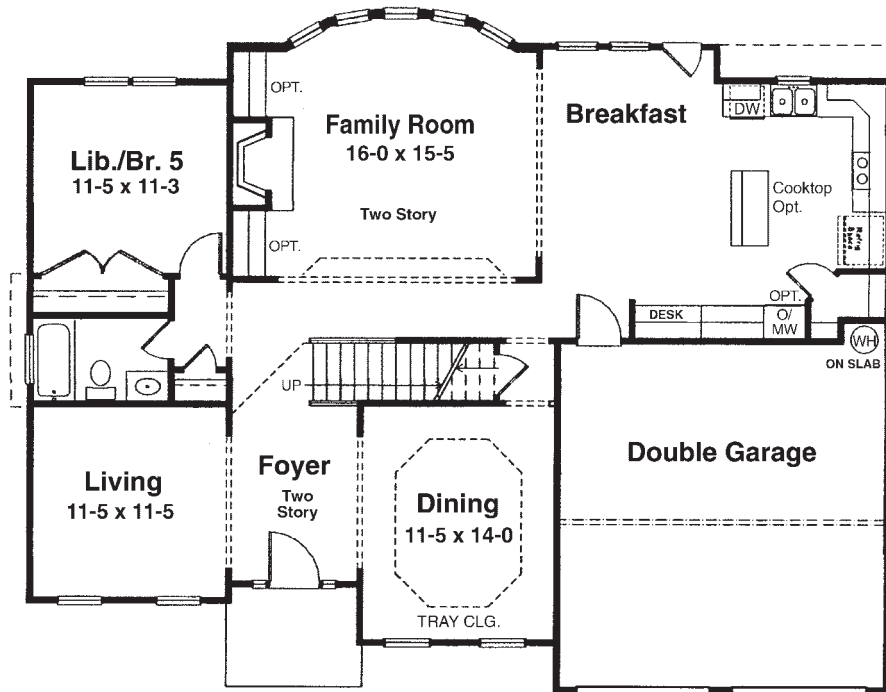
ELEV. "A" FIRST FLOOR
