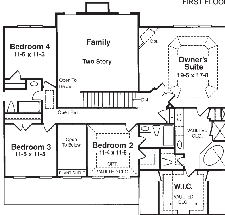
ELEV. "C" FIRST FLOOR
