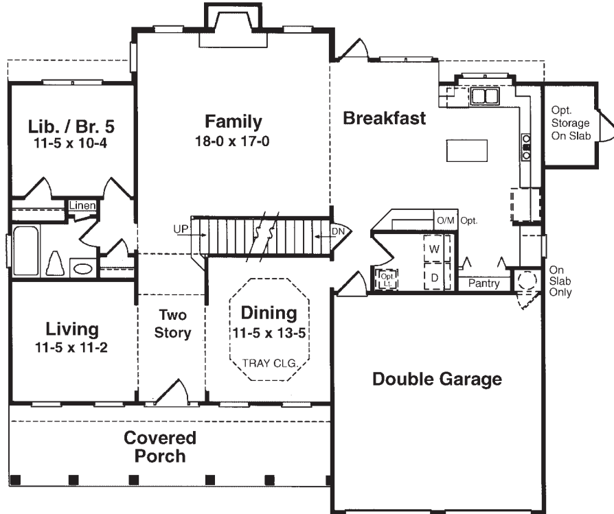
ELEV. "C" FIRST FLOOR
